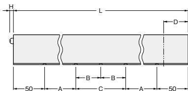
No.558-1LW、No.558-2LS、No.558-2LW
